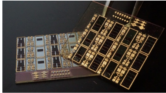
Integrated Passive Device Matching Network from 3D Glass Solutions
